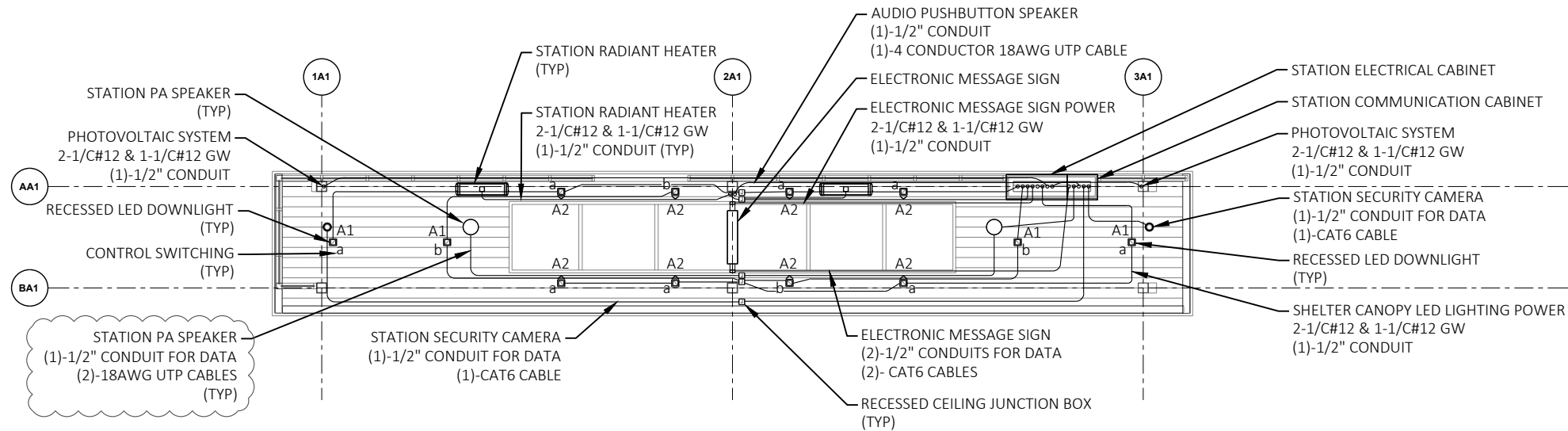
PLATFORM - CEILING PLAN
