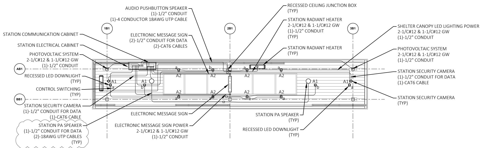
PLATFORM - CEILING PLAN
