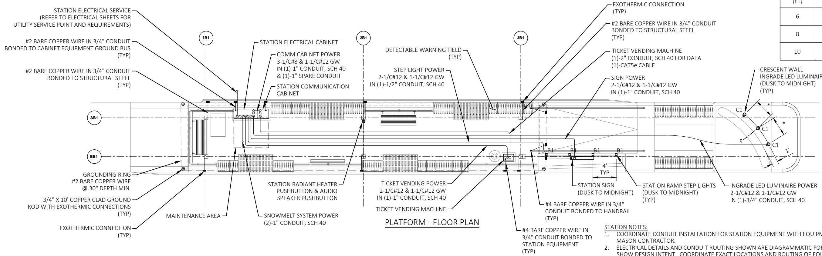
TYPICAL CENTER STATION PLATFORM ELECTRICAL DETAILS (TYPE "B" PLATFORMS)
